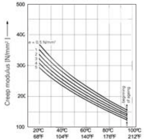
Figure D-5. Creep modulus curve for PPH at 10 years
