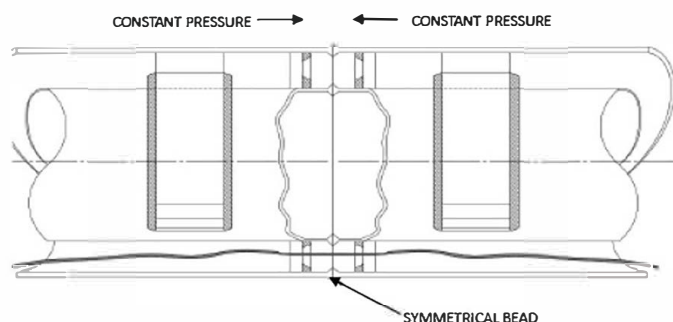
Figure 4: Welding complete with pull rope installed
