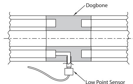
Figure G-19. Simple connection, Duo-Pro® Fluid-Lok® systems
