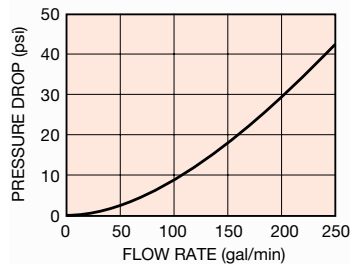
2 x 3 Inch Pipe
