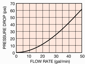
1 x 2 Inch Pipe
