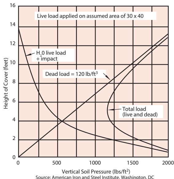
Figure G-3. H 2 O highway loading
