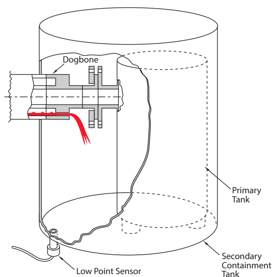
Figure G-21. End-of-line connection option, Duo-Pro®/Fluid-Lok® systems
