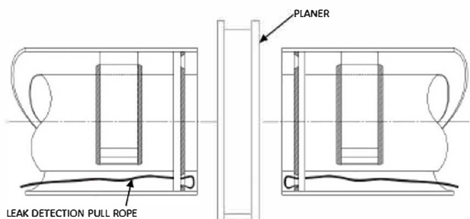
Figure 1: Planing ends with pull rope installed
