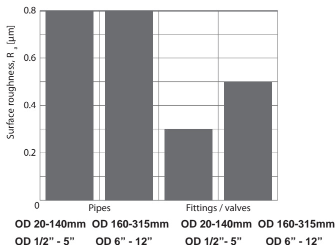
Figure D-15. Surface specification for PP-Pure® pipes
