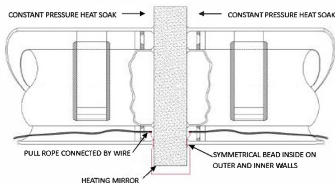
Figure 3: Pipe ends heated with pull rope installed
